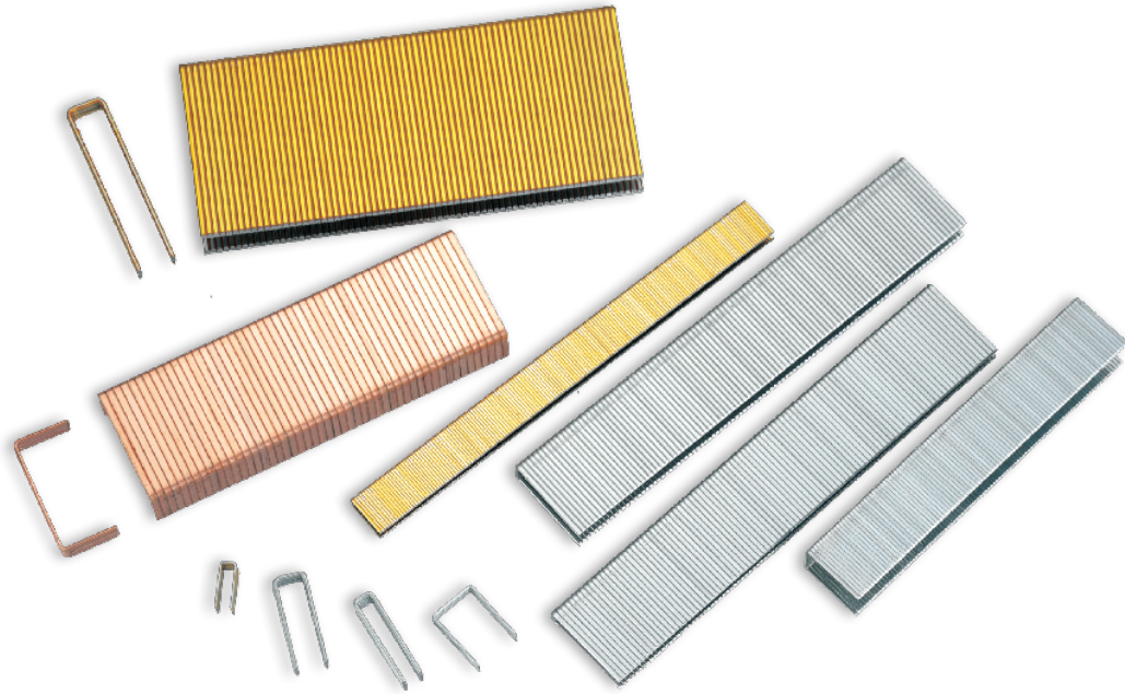
Fine Wire / Medium Wire / Heavy Duty Staples From 12-23GA.
