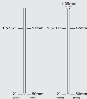
23GA. \varnothing 0.84mm
