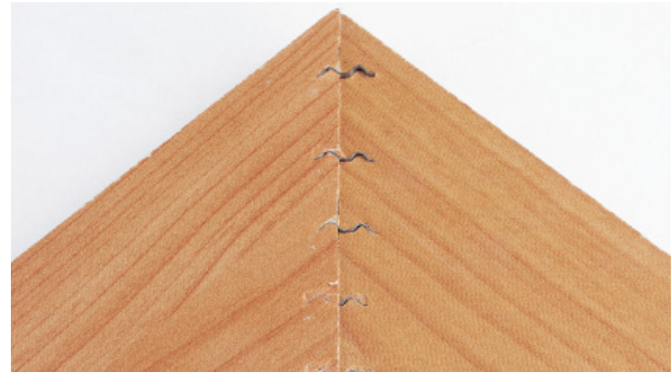
Butt Joints. Inside Mitres. Outside Mitres, Picture Frames and Face Frames
