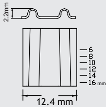
MCF127 NAILS SPEC.
