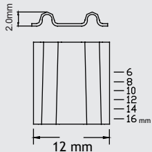
SCF16 NAILS SPEC.
